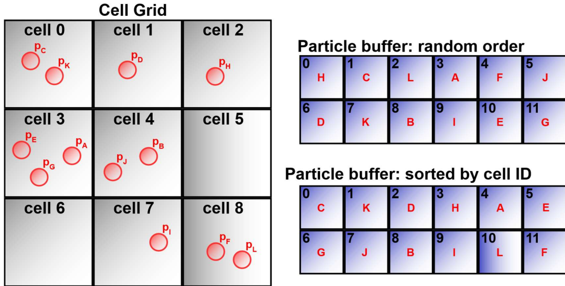
Figure 6: Unsorted vs sorted particle data in memory.
