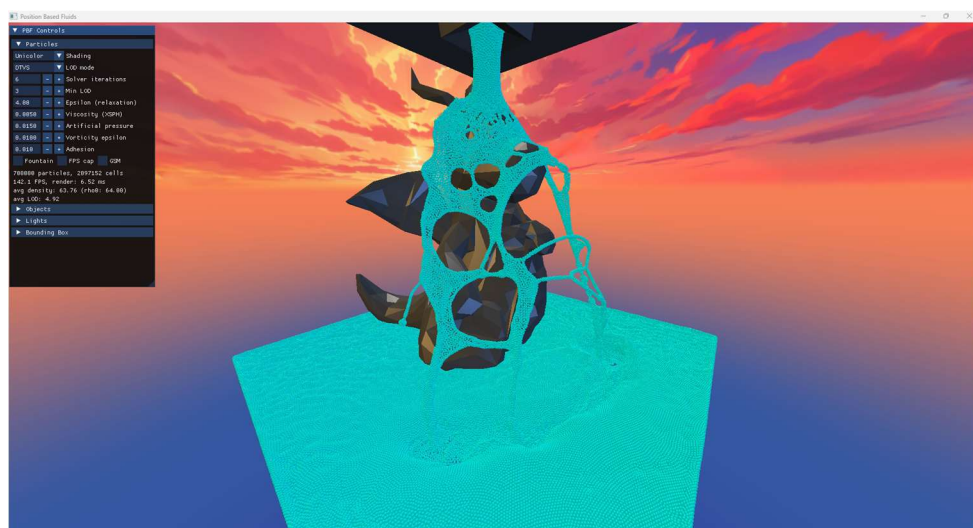
Figure 17: Unicolor shading.
