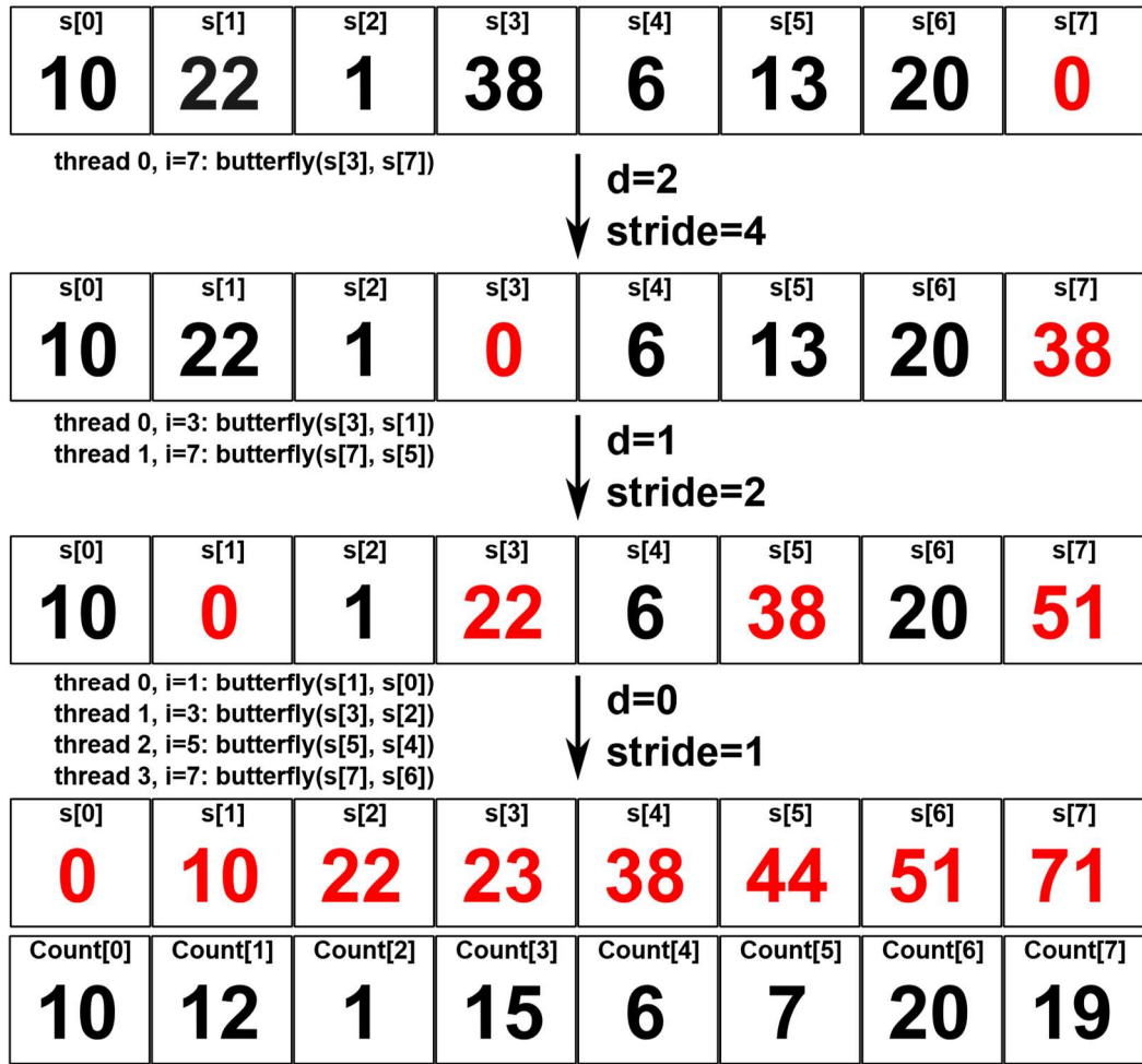
Figure 10: Blleloch scan down-sweep array visualization.
