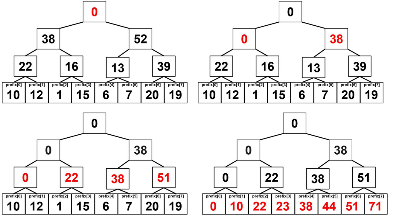
Figure 12: Blleloch scan down-sweep tree visualization.
