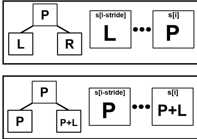
Figure 8: Blleloch scan butterfly.
